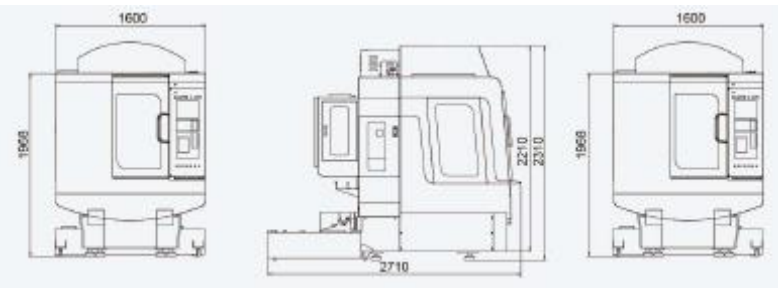
TMV-510CII
