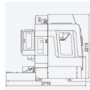
TMV-510AII
